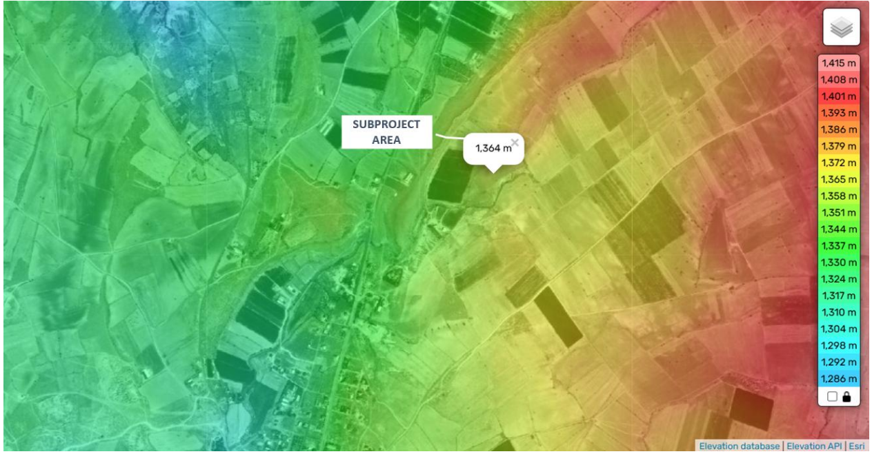
Figure 6. Topographic Map
