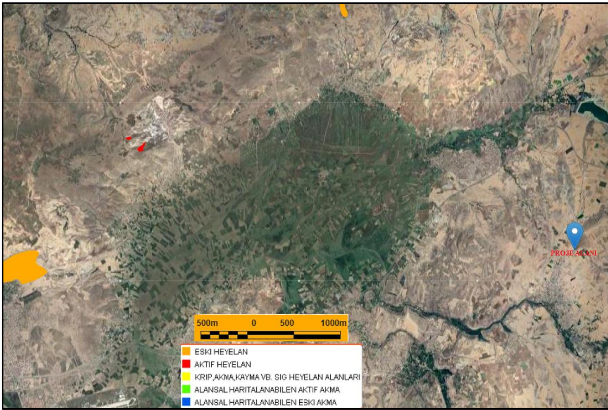
Figure 10. Landslide Map 3
